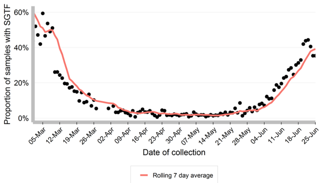
Figure 16. Proportion of samples with S gene target failure (SGTF), 1 March 2022 to 25 June 2022
